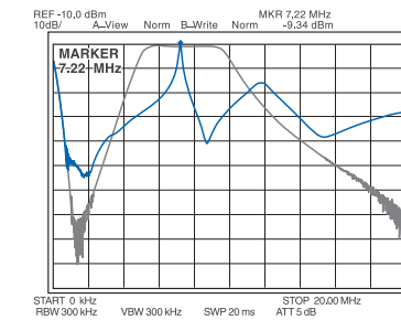
■ BPF and preselector passband characteristics receiving on 7.22 MHz
